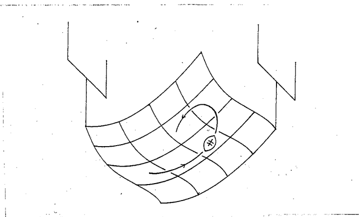
Figure 2: Complex integration and american football.
