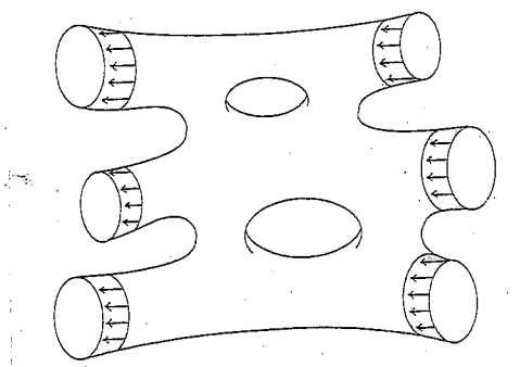
Figure 1: The Residue Theorem as a Conservation Law.
