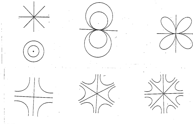
Figure 3: Zeros and poles of meromorphic vector fields.
