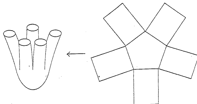
Figure 4: Construction of a differential form with prescribed residues.
